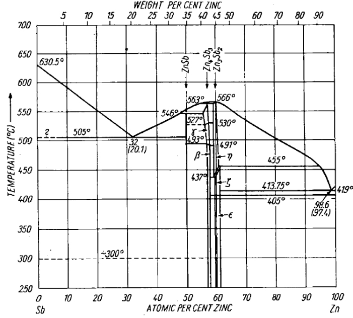
Figure 1.3: Zn-Sb phase diagram. Reproduced from Ref. [16].
