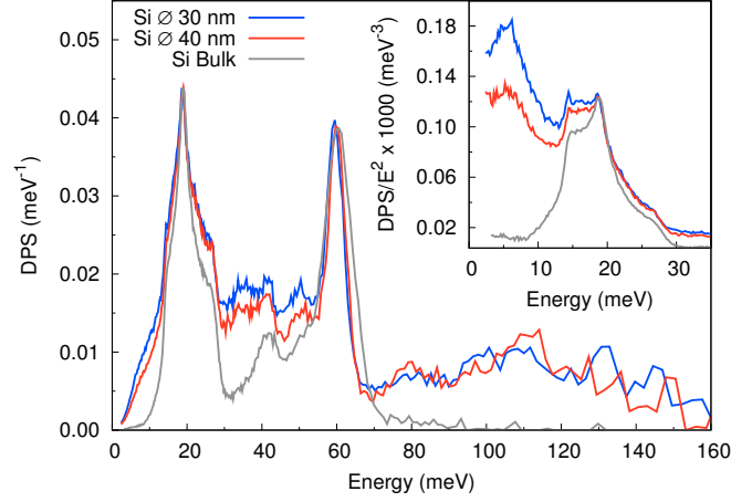
Figure 2.4: Density of Phonon States (DPS) for both nanocrystalline Si compared with reference polycrystalline Si. Inset: the reduced DPS, where the Boson peak around 6 meV is a clear indication of amorphous \text{SiO}_2 .
